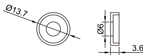
Washer
