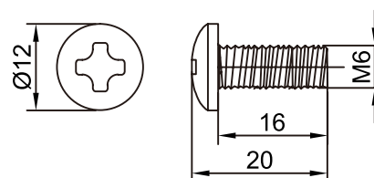
Screw
